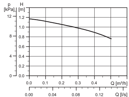
Grundfos COMFORT 15-14 B[A] PM Grundfos COMFORT 15-14 MB PM
